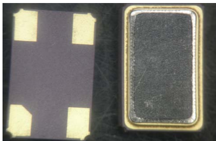
SMD6035 (6.0*3.5mm)
